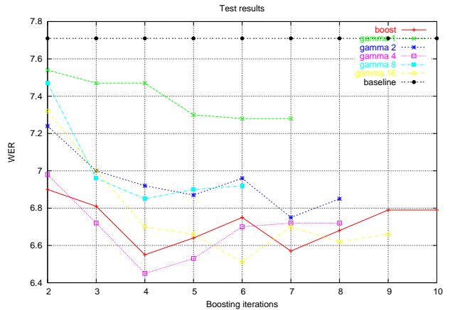
Fig. 2. Test word error rates for various values of gamma, compared with a baseline system and the previous boosting approach.
