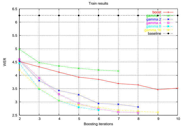
Fig. 1. Training word error rates for various values of gamma, compared with a baseline system and the previous boosting approach.
