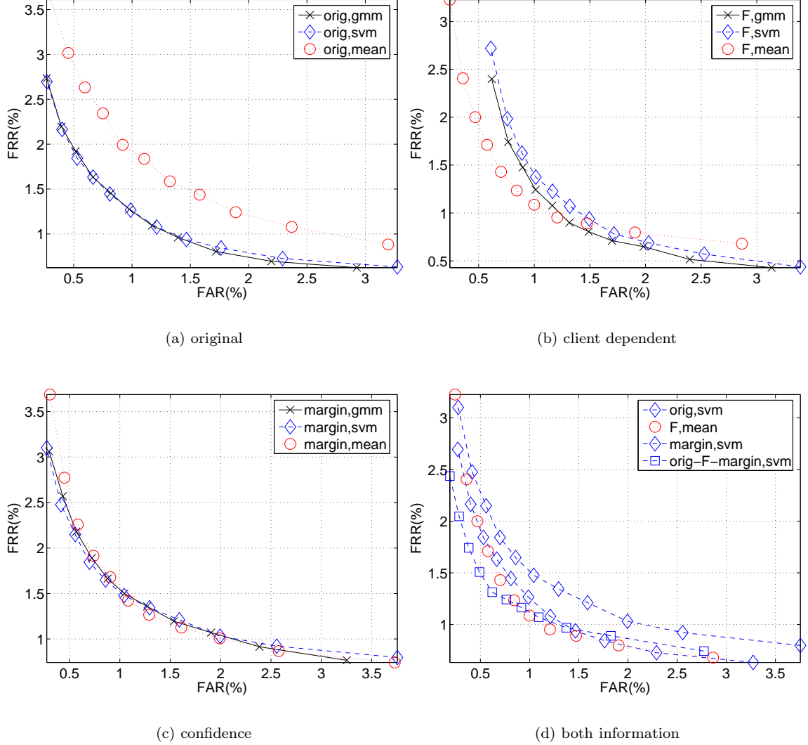
Figure 2: Pooled ROC curves from 32 XM2VTS benchmark fusion data sets of three baseline experiments (a)–(c) and fusion with all information sources (d). (a) is fusion with the original scores, \{y_i|\forall_i\} , (b) is fusion with F-ratio transformed scores, \{y_i^F|\forall_i\} , and (c) is fusion with margin-derived confidence, \{y_i q_i|\forall_i\} , each using a GMM, an SVM with linear kernel and the mean operator. The “best” three pooled ROC curves (i.e., the EPC curve with the lowest HTER value across different \alpha values) in (a)–(c) are plotted in (d), together with the one that fuses all sources of information, i.e., \{y_i, y_i q_i, y_i^F|\forall_i\} using an SVM with linear kernel, denoted as “orig-F-margin,SVM”. This figure complements Figure 1. As confirmed by the HTER significance test, for FRR above 1.2%, “orig-F-margin,SVM” is significantly different (and better) than “F-mean” but below 1.2%, their difference is insignificant . This phenomenon is due to few client accesses as compared to impostor accesses. As a result, low FRR values cannot be interpreted reliably compared to low FAR values.
