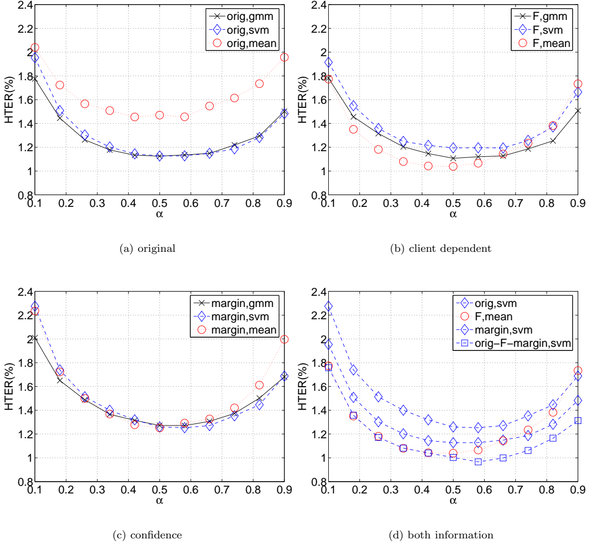
Figure 1: Pooled EPC curves from 32 XM2VTS benchmark fusion data sets of three baseline experiments (a)–(c) and fusion with all information sources (d). (a) is fusion with the original scores, \{y_i|\mathcal{V}_i\} , (b) is fusion with F-ratio transformed scores, \{y_i^F|\mathcal{V}_i\} , and (c) is fusion with margin-derived confidence, \{y_i q_i|\mathcal{V}_i\} , each using a GMM, an SVM with linear kernel and the mean operator. The best three pooled EPC curves in (a)–(c) are plotted in (d) (the top three in the legend), together with fusion with all sources of information, i.e., \{y_i, y_i q_i, y_i^F|\mathcal{V}_i\} using an SVM with linear kernel, denoted as “orig-F-margin,SVM”. The pooled EPC of this curve is compared to the “best overall fusion” (lowest HTER in the EPC curve across different \alpha ) in each of (a)–(c). “orig-F-margin,SVM” is better than “F-mean” for \alpha > 0.6 according to the HTER significance test at 90% of confidence. Below \alpha > 0.6 , both EPC curves are not significantly different .
