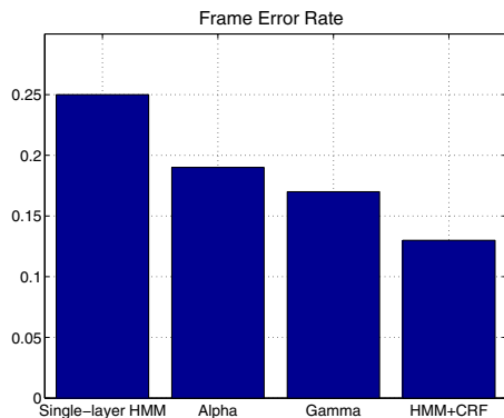
Fig. 4. Comparison of the four methods – the single-layer HMMs, the multi-layer approach based on \alpha , \gamma , and CRFs – in terms of FER ( frame error rate ).
