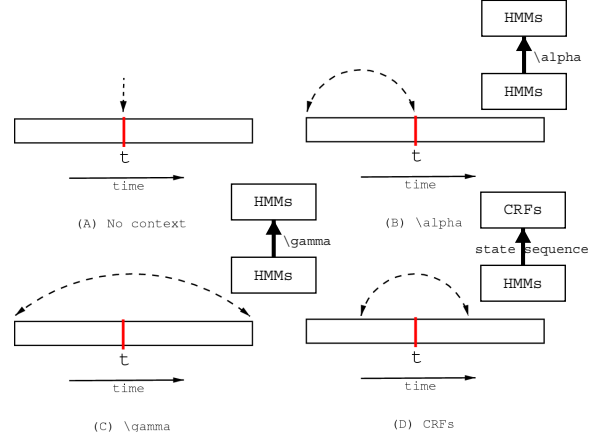
Fig. 2. Illustration of context information (Note that t indicates the current time): (A) without contextual information; (B) “Alpha” taking into account the contextual information of the past observation from the beginning up to the current time X_1^t ; (C) “Gamma” taking into account the contextual information of the whole observation X_1^T ; (D) Conditional random field taking into account the arbitrary contextual information.
