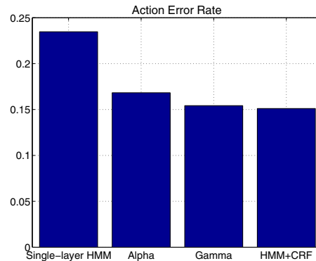
Fig. 5. Comparison of the four methods – the single-layer HMMs, the multi-layer approach based on \alpha , \gamma , and CRFs – in terms of AER ( action error rate ).
