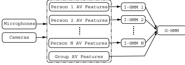
Fig. 1. The multi-layer framework applied to group action recognition: the lower layer recognizes individual actions of participants using low-level audio-visual (AV) features. The output of this layer provides the input to the second layer, which models interactions. Individual actions naturally constitute the link between the low-level audio-visual features and high-level group actions.
