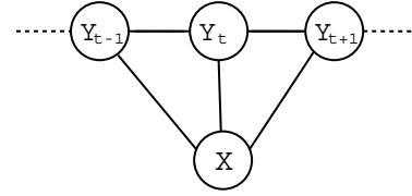
Fig. 3. Conditional Random Fields: the hidden nodes can depend on observations at any time step, thus relaxing the independence assumptions required by HMMs.
